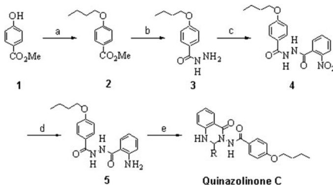
Fig. 1. The synthetic route of quinazolinone C. Reagents and conditions: a, 1: NaOH, MeOH, 0°C, 20 min; 2: n -BuBr, MeOH, reflux, 5 h; b, N 2 H 4 ·H 2 O, MeOH, reflux, 6 h; c, 2-nitrobenzoyl chloride, Et 3 N, CH 2 Cl 2 , 0°C to room temperature, overnight; d, Zn, AcOH, CH 2 Cl 2 , 0°C to room temperature, 4 h; e, substituted benzaldehyde, AcOH/ N,N -dimethylacetamide/CH 2 Cl 2 (5:5:90), 4A molecular sieve, reflux, 12 h.
