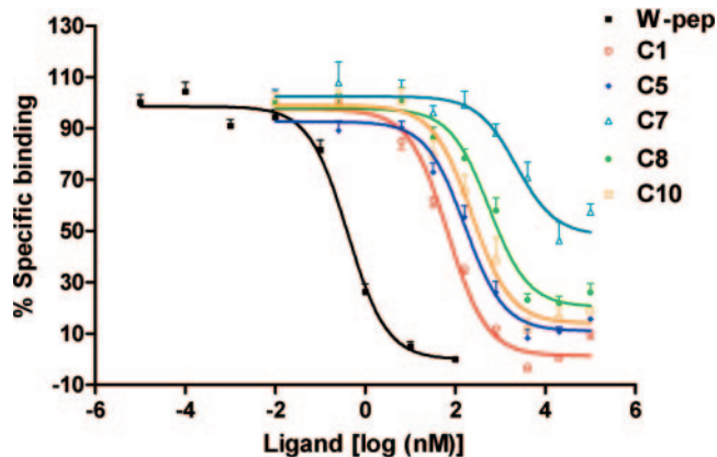
Fig. 6. Competitive binding of selected C series derivatives to [^{125}I] WKYMVm with FPRL1. Cell membrane was prepared from RBL-FPRL1 cells. Various concentrations of compounds were incubated together with RBL-FPRL1 cell membrane preparation, 0.16 nM [^{125}I] WKYMVm, and FlashBlue GPCR beads. The plates were incubated at 4°C for 12 h and centrifuged for 3 min at 2500g before counting on a MicroBeta scintillation counter. The results (means \pm S.E.M.) are expressed as the percentage of specific binding from three independent experiments.
