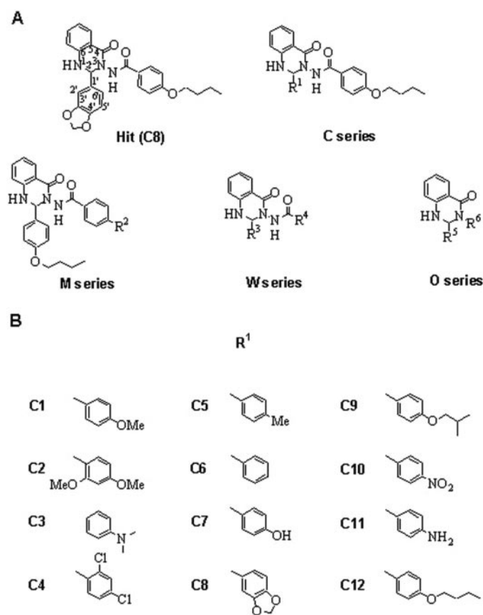
Fig. 2. Chemical structures of hit compound (C8) and its derivatives. A, structure of the hit compound identified from high-throughput screening and its four series derivatives (C, M, W, and O). B, structures of C series derivatives at R 1 . Compound C1 is the previously reported FPRL1 agonist Quin-C1. Derivatives were designed based on hit compound C8 by changing the substitution on the phenyl group at the 2 position while keeping the basic quinazolinone skeleton.
